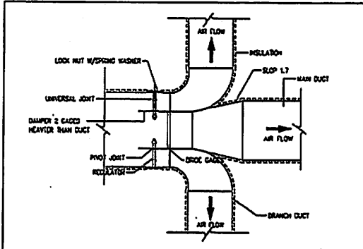
BRANCH TAKE-OFF WITH SPLITTER DAMPER
