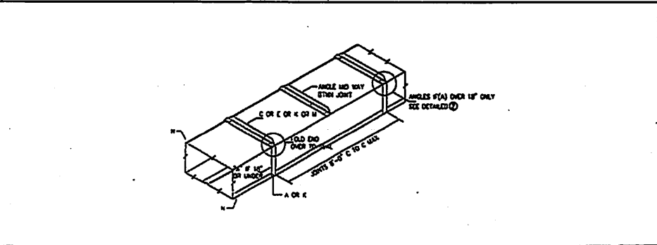
DUCT 19" THRU 30"
