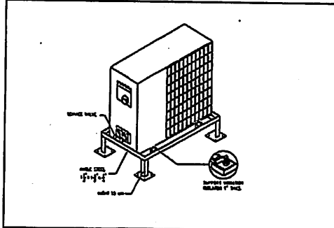
INSTALLATION OF CONDENSING UNIT
