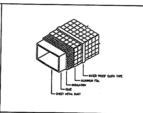
DUCT INSULATION
