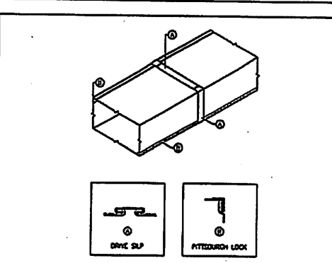
DUCT CONSTRUCTION DETAILS
