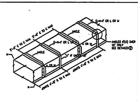
DUCT 61" THRU 84"
