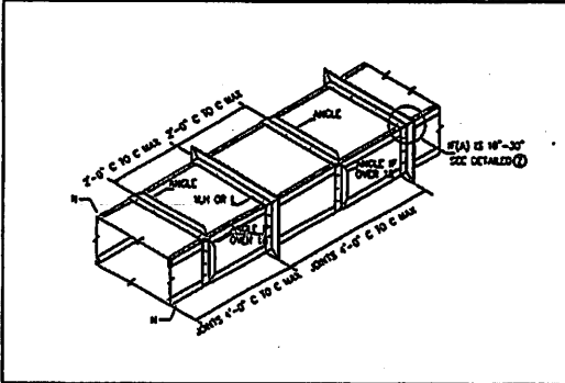
DUCT 85" AND OVER
