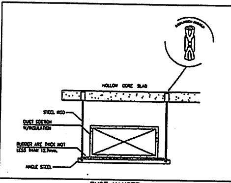
DUCT HANGER
