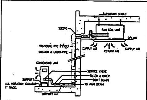
INSTALLATION OF AIR CONDITIONER (CASSETTE TYPE)
