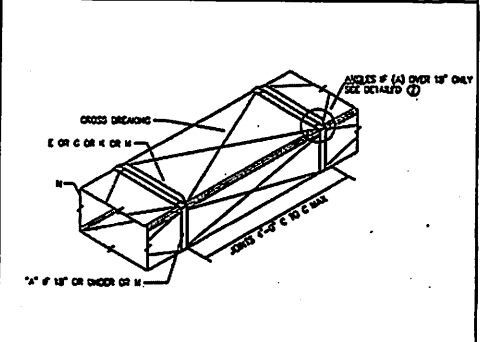
DUCT 31" THRU 60" (CONSTRUCTION WITH CROSS BREAKING)
