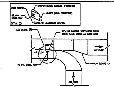
BRANCH TAKE-OFF FOR SUPPLY AIR DUCT
