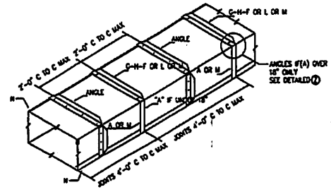
DUCT 61" THRU 84"
