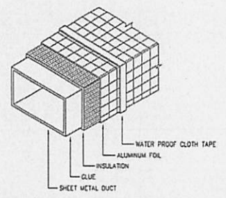
DUCT INSULATION
