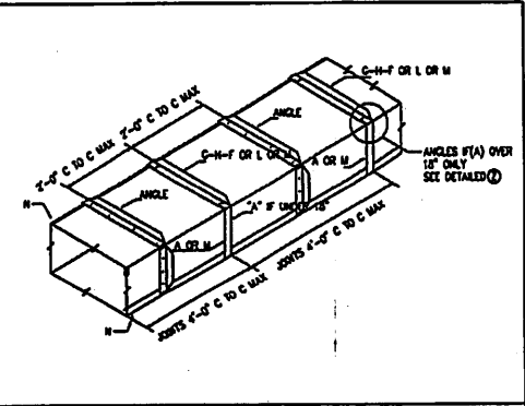
DUCT 61" THRU 84"
