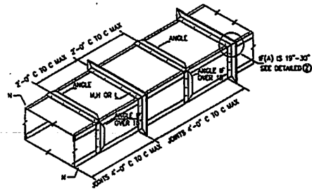
DUCT 85" AND OVER
