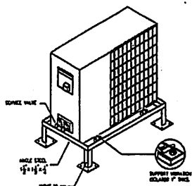
INSTALLATION OF CONDENSING UNIT
