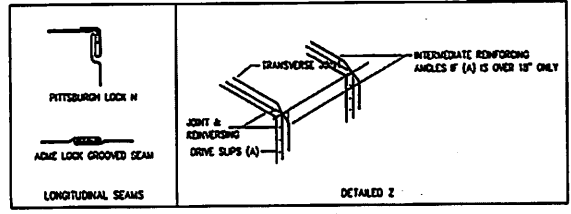
DETAILED Z
