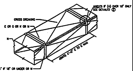
DUCT 31" THRU 60" (CONSTRUCTION WITH CROSS BREAKING)
