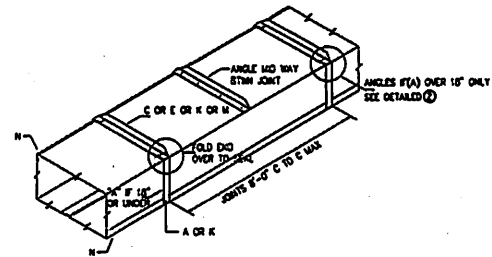
DUCT 19" THRU 30"
