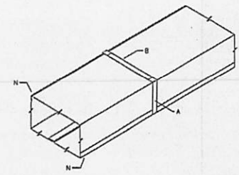
DUCT THRU 18" MAXIMUM DIMENSION
