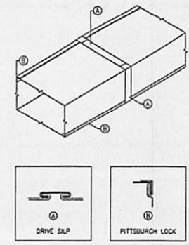
DUCT CONSTRUCTION DETAILS
