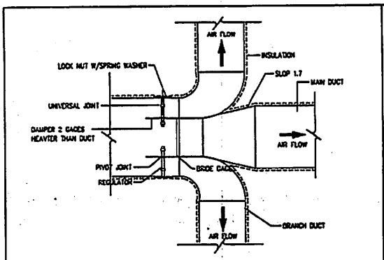
BRANCH TAKE-OFF WITH SPLITTER DAMPER
