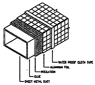
DUCT INSULATION
