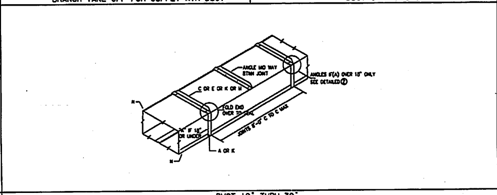
DUCT 19" THRU 30"
