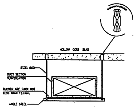
DUCT HANGER
