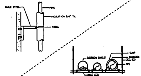
PIPE HANGER
