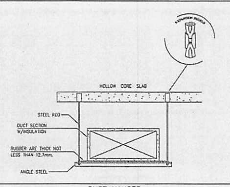
DUCT HANGER
