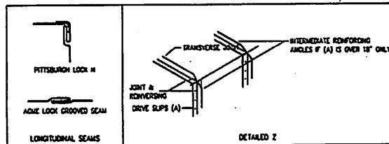
DETAILED Z
