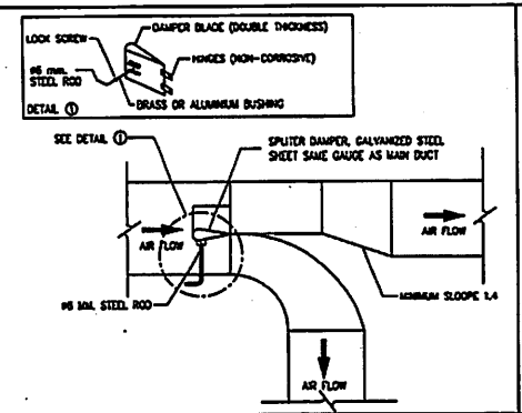
BRANCH TAKE-OFF FOR SUPPLY AIR DUCT
