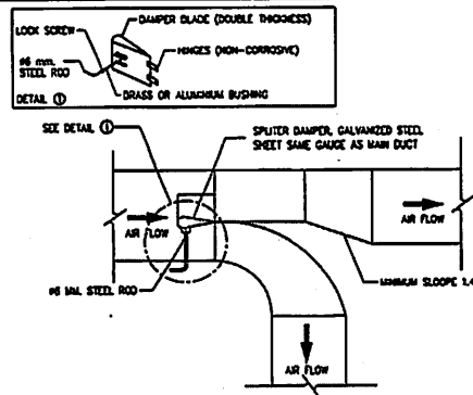
BRANCH TAKE-OFF FOR SUPPLY AIR DUCT
